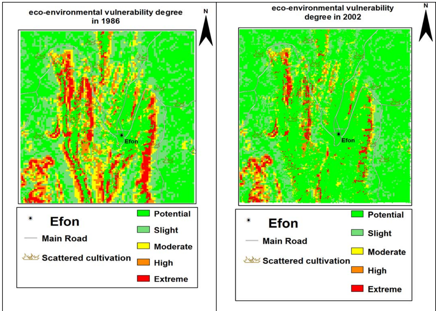
Figure 7: Distribution of eco-environmental in study area, showing the eco-environment vulnerability level in 1986 and 2002, respectively, as well as a general change trend since the green region standing for "potential" is expanding gradually from 1986 to 2002.
