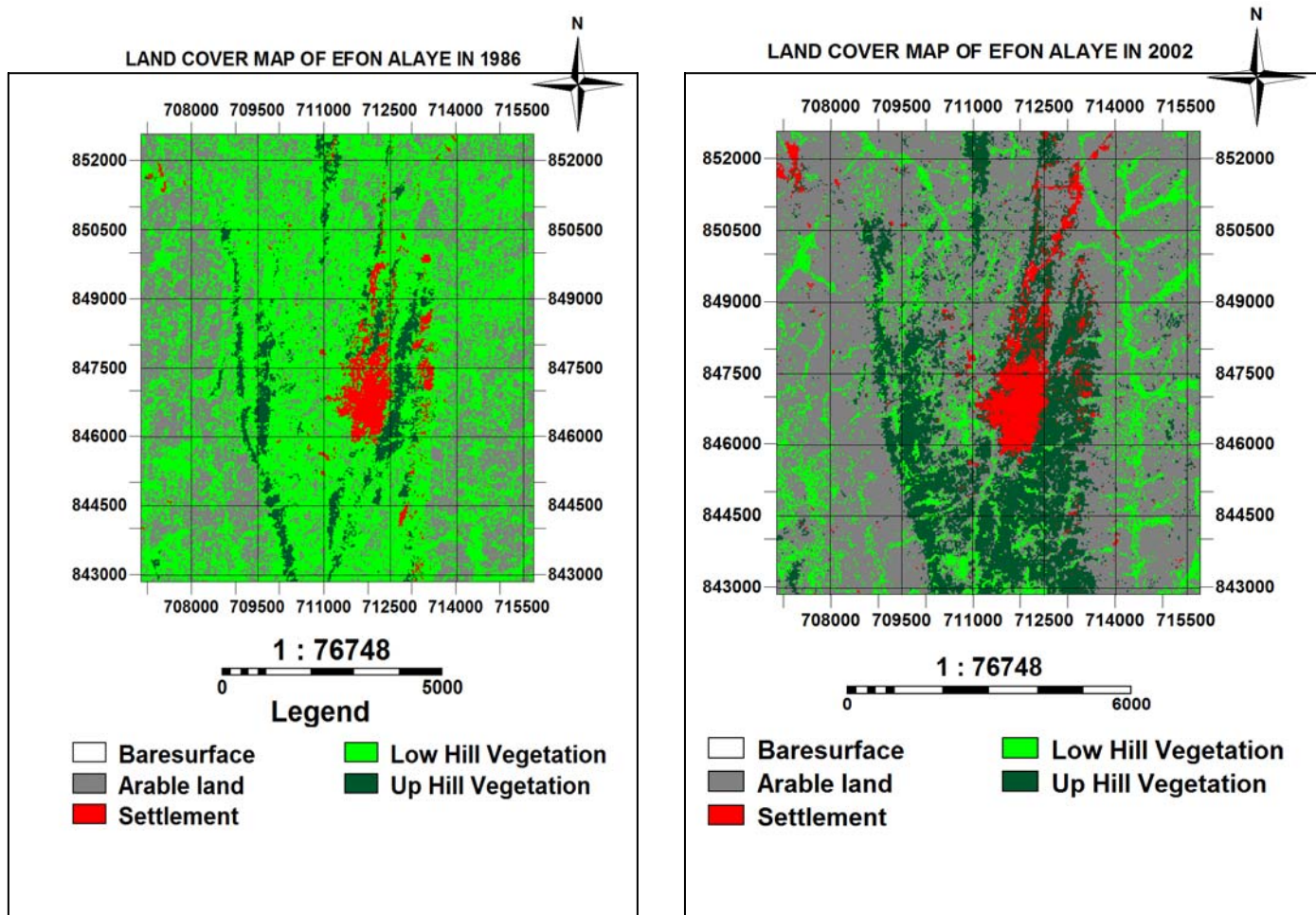
Figure 2: Land use/ Land cover classification of the study area in 1986 and 2002
