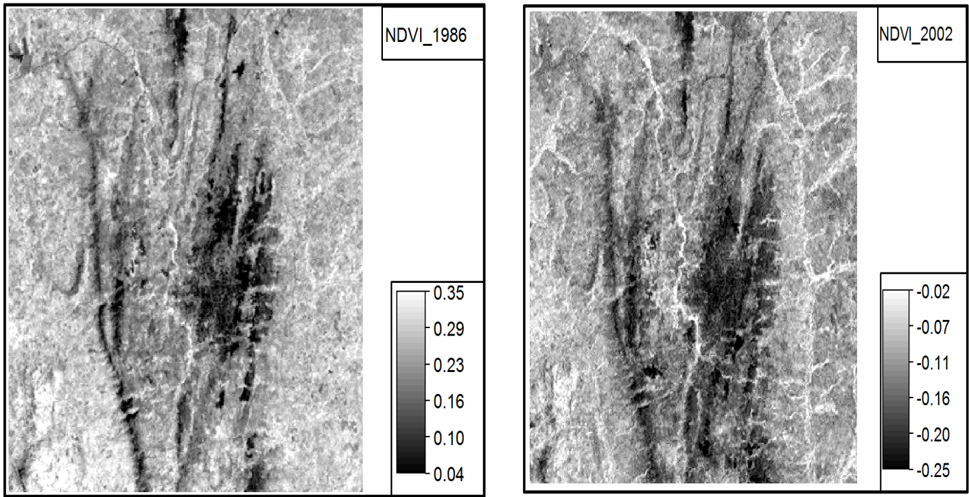
Figure 4: Image representation of Vegetation Map (NDVI) of 1986 and 2002
