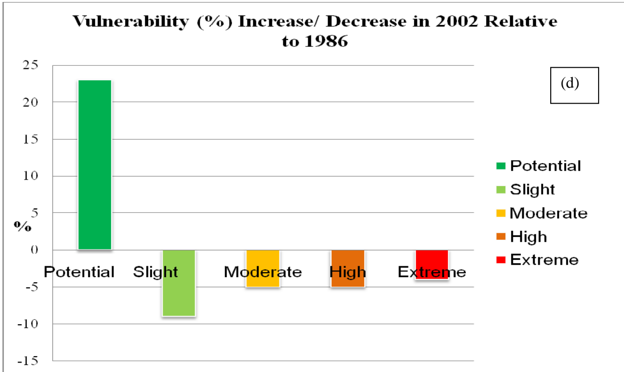
Figure 8: (a) - (d) Change of eco-environmental vulnerability between 1986 and 2002.
